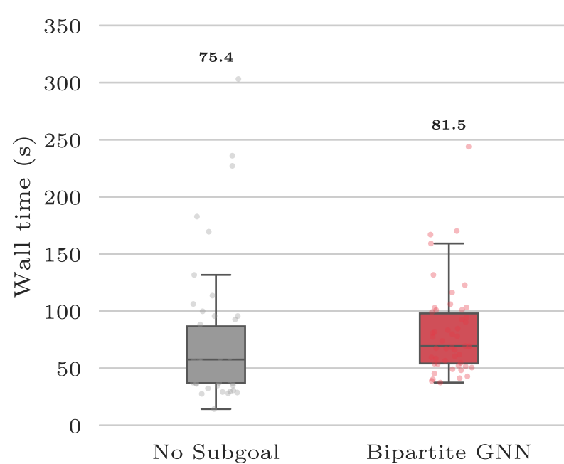
OMPL Wall Time
