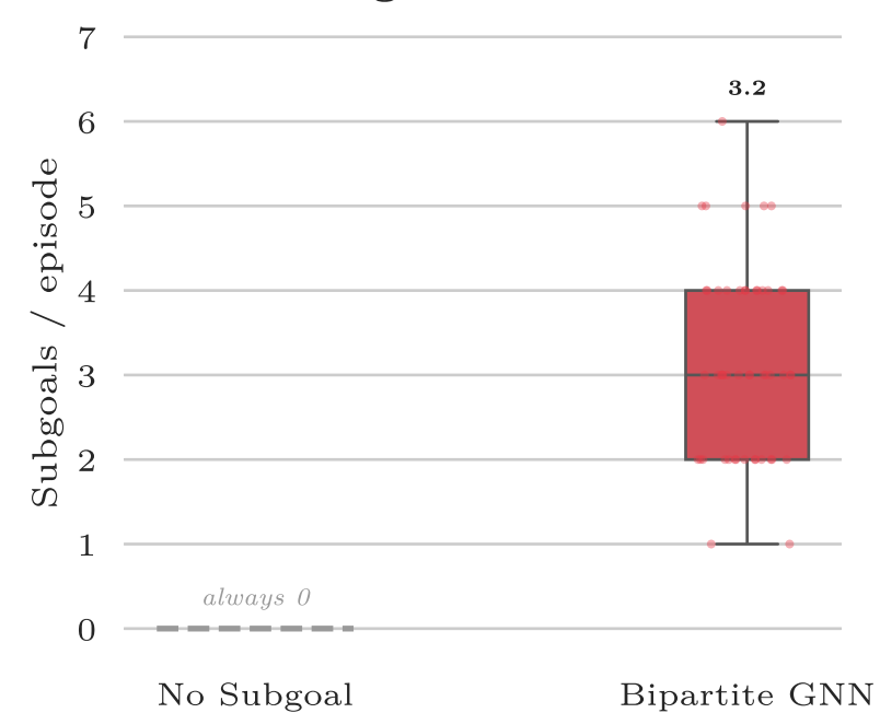
Subgoals Reached
