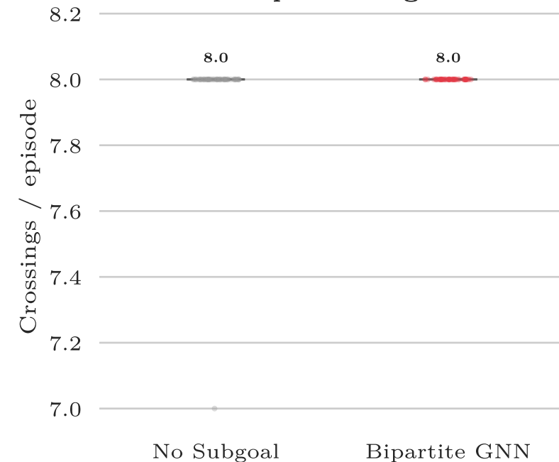
Gap Crossings
