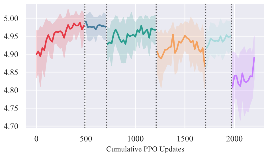
Mean Crossings
