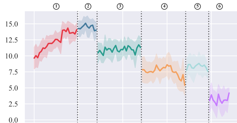
Mean Reward
