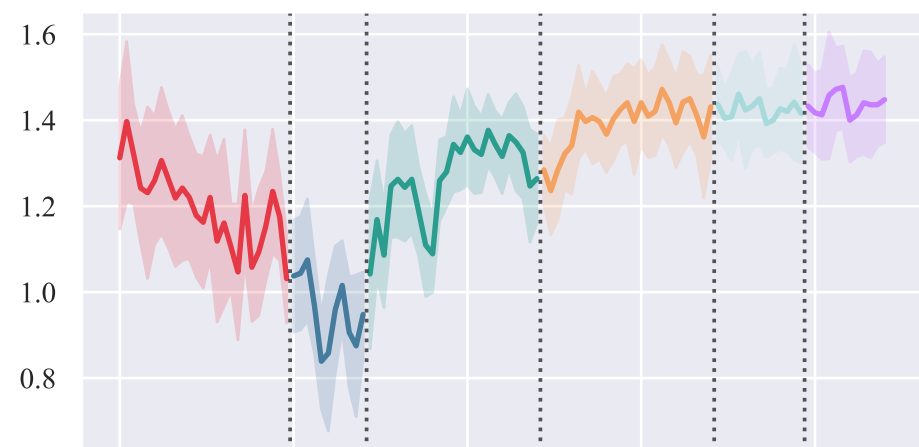
Skipped Subgoals
