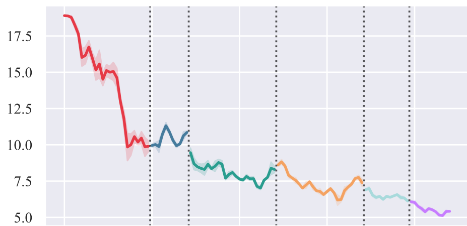
Position Entropy
