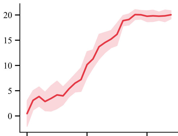
Mean Reward
