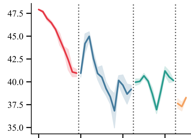
Position Entropy
