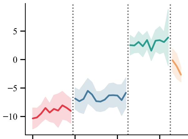
Mean Reward
