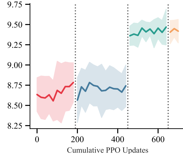
Mean Crossings
