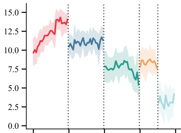
Mean Reward
