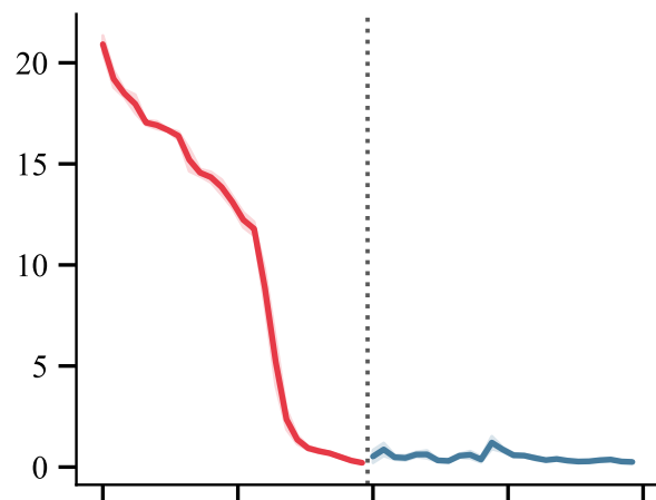
Position Entropy
