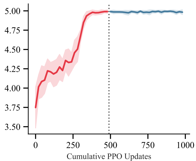
Mean Crossings
