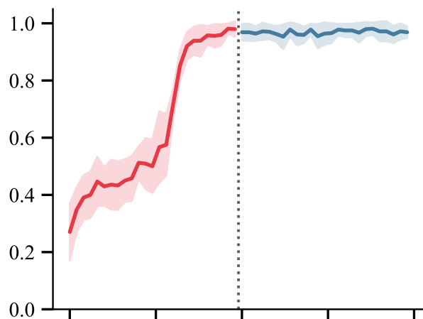
Frac. Terminated
