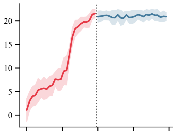
Mean Reward
