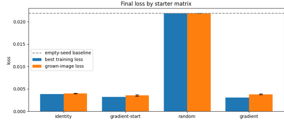
Figure 15: In averaged loss after growing a full lizard from a pixel, the random matrix start sits at the empty baseline. Identity comes third place at 0.0040, gradient-only is second at 0.0038 (+/- 0.000086) and the best result comes from further training the gradient output with CMA-ES at 0.0036 (+/- 0.000177).
