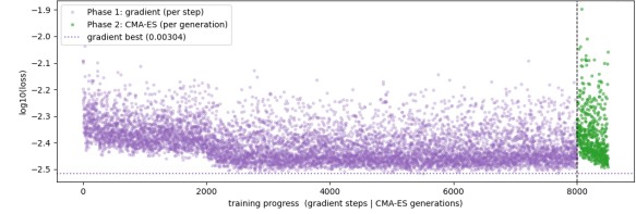
Figure 13: CMA-ES does not visibly improve upon the gradient-baseline training loss within 500 generations. There is a significant jump upwards in loss after the switch, likely caused by sigma0 being too high and too big changes being made.
