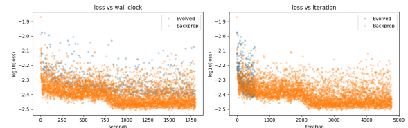
Figure 6: Different ways of measuring the x-axis: time or training steps/generations. On the y-axis, the loss of the gradient-approach is always a bit better (lower) than the evolved one. Comparing by training steps/generation, the losses look comparable, though much more computational steps are completed per generation than per training step, making the time-based measurement approach the 'fairest' one.
