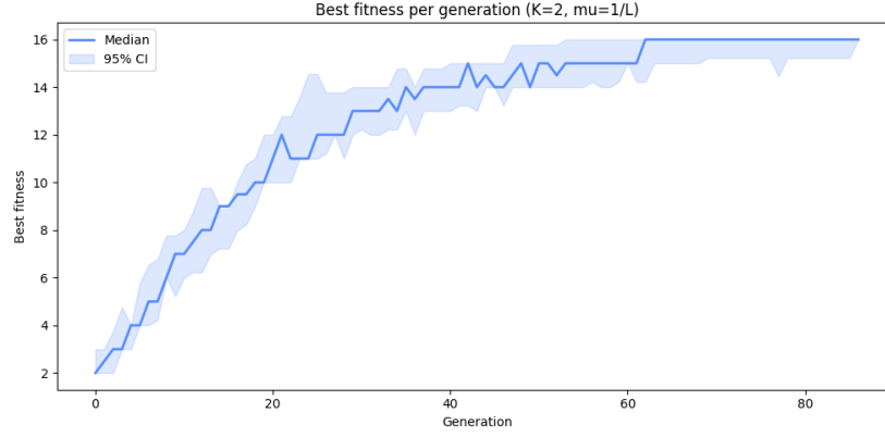
Figure 1: Results of running the GA 10 times with baseline values ( K = 2 , \mu = 1/L , N = 200 ). The blue line shoes the median over 10 samples, while the light blue shaded area shows the confidence interval.
