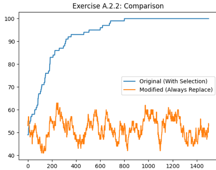
Figure 11: Fitness against generations.
