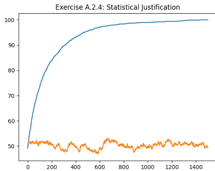
Figure 12: Averages of fitness vs generations across multiple runs.
