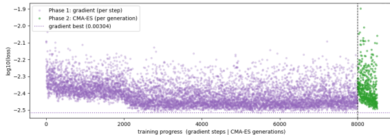
Figure 15: CMA-ES does not visibly improve upon the gradient-baseline training loss within 500 generations. There is a significant jump upwards in loss after the switch, likely caused by sigma0 being too high and too big changes being made.
