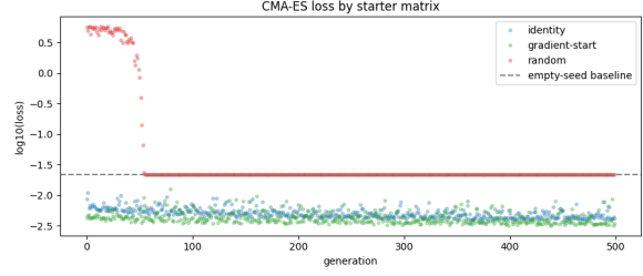
Figure 16: While the model trained starting from the identity matrix and the model trained from the gradient-result-matrix continued improving, the white-noise matrix start only managed to not be worse than producing a white canvas and got stuck there. The baseline here is the loss for the starter image of white canvas with a single black pixel in the middle.
