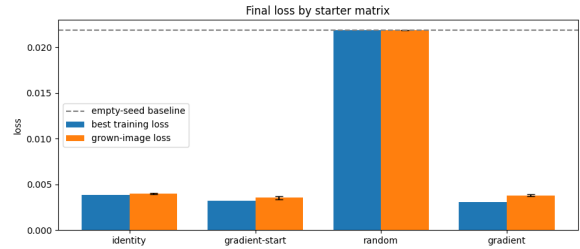
Figure 17: In averaged loss after growing a full lizard from a pixel, the random matrix start sits at the empty baseline. Identity comes third place at 0.0040, gradient-only is second at 0.0038 (+0.000086) and the best result comes from further training the gradient output with CMA-ES at 0.0036 (+0.000177).
