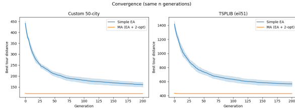
Figure 5: Distance vs n Generations, with the mean in blue/orange and the standard deviation in light blue/orange over 10 samples.
