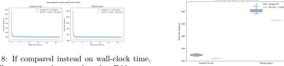
Figure 9: While the gap has shrunk considerably from comparing by number of generations, MA still provides better and more consistent results than EA.
