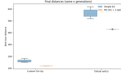
Figure 6: Best distance of EA and MA on both datasets.
