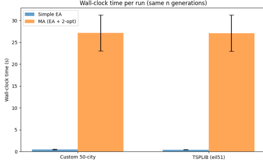
Figure 7: Time comparison between EA and MA both running for 200 generations, mean score over 10 runs.
