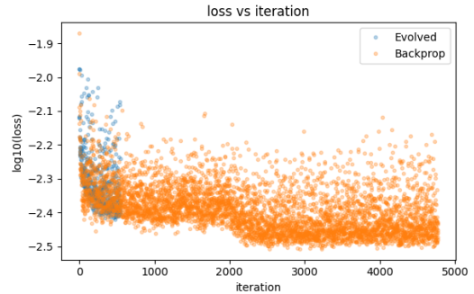
Figure 7: Optimization trajectory measured by training iterations.
