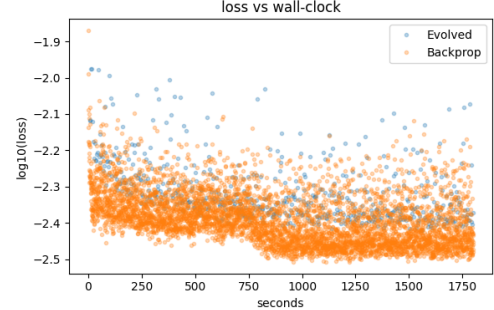
Figure 6: Optimization trajectory measured by wall-clock time (approximately 30 minutes).
