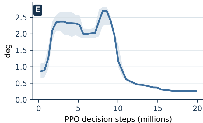
Vehicle tilt
