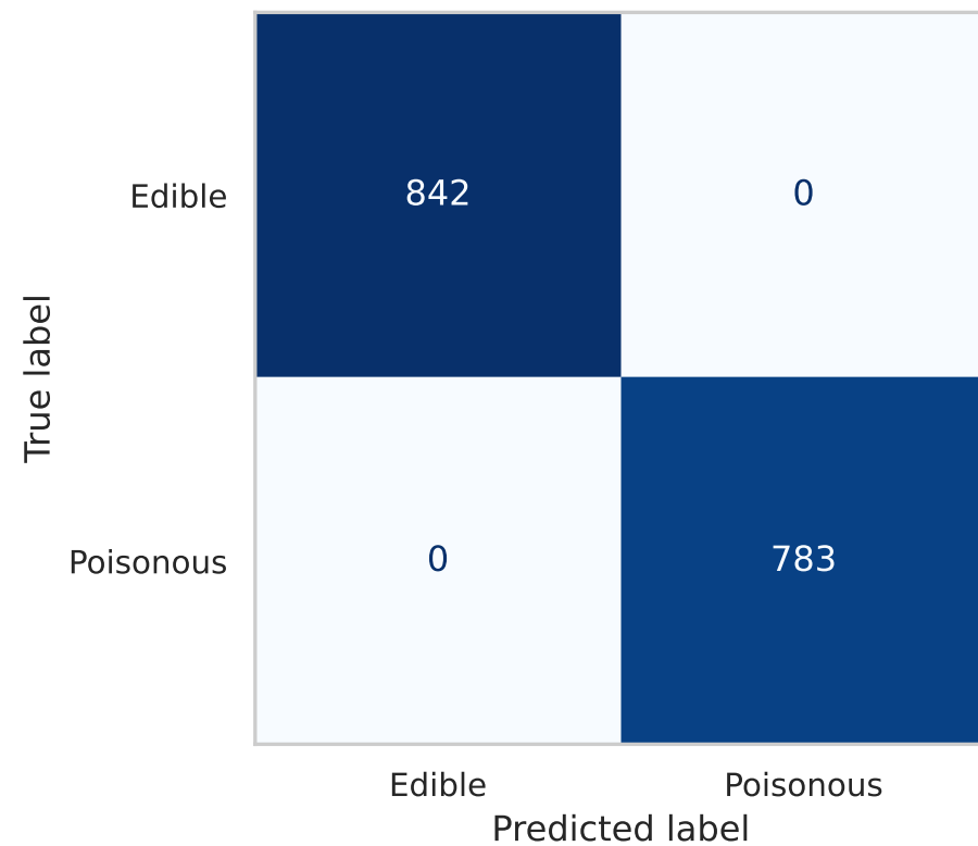
XGBoost
