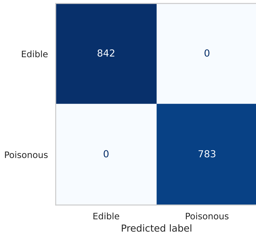
Decision Tree
