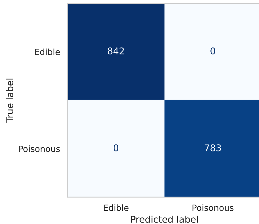
Random Forest
