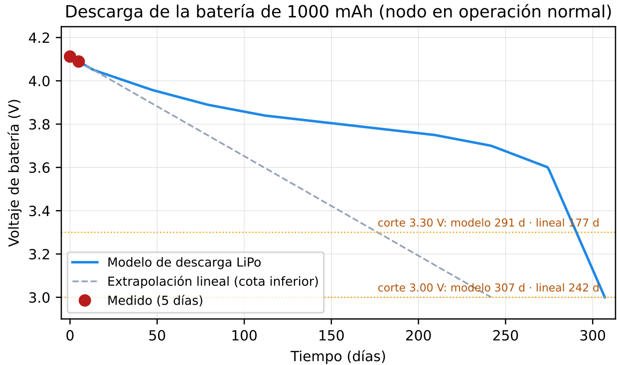
Figure 6: Two measured voltage points over five days with a 1000 mAh cell and extrapolated curves. Estimated autonomy is 177 days (linear, 3.30 V cutoff) or 291–307 days (assumed LiPo curve, 3.30/3.00 V cutoffs). The original plot’s lower-bound label compares models; it does not guarantee service lifetime.
