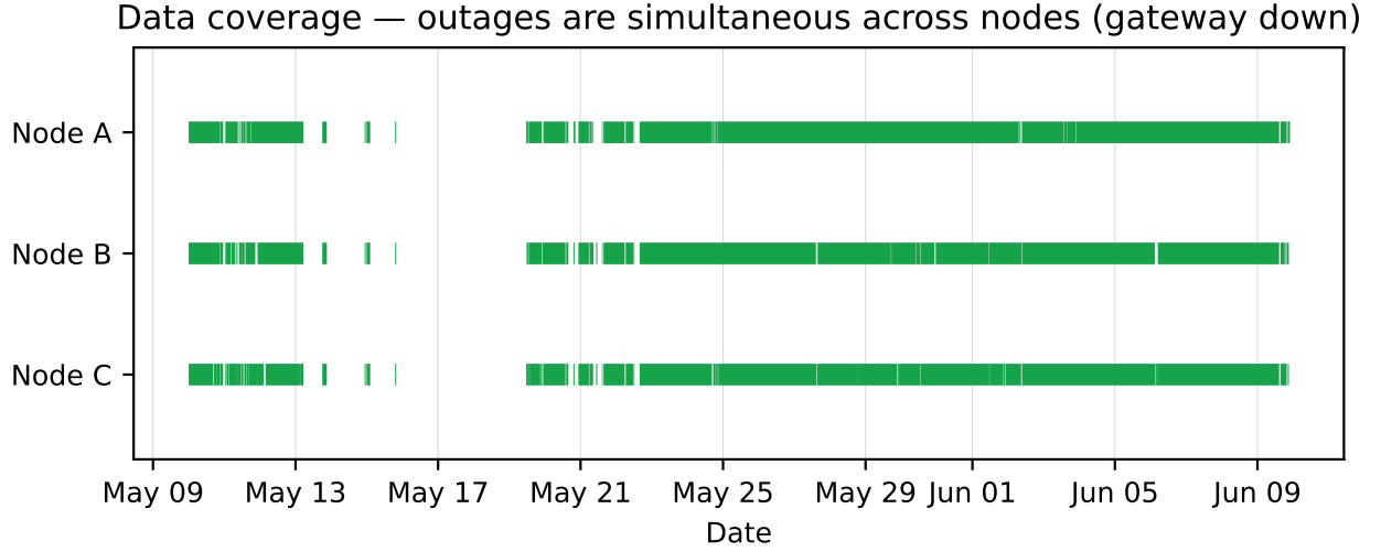
Figure 8: Data coverage in the three-node overlapping interval. White gaps retain missing data. The original “gateway down” plot label is an interpretation compatible with simultaneous interruptions, not an independently verified power-state record.
