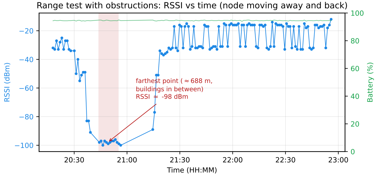
Figure 3: Urban obstructed-path test of 20 August 2026: per-packet RSSI (blue) and voltage-derived battery indication (green) against time during a mobile outward and return route. The link remained operational near 688 m at approximately -98 dBm; distance was not a controlled fixed-position sweep.
