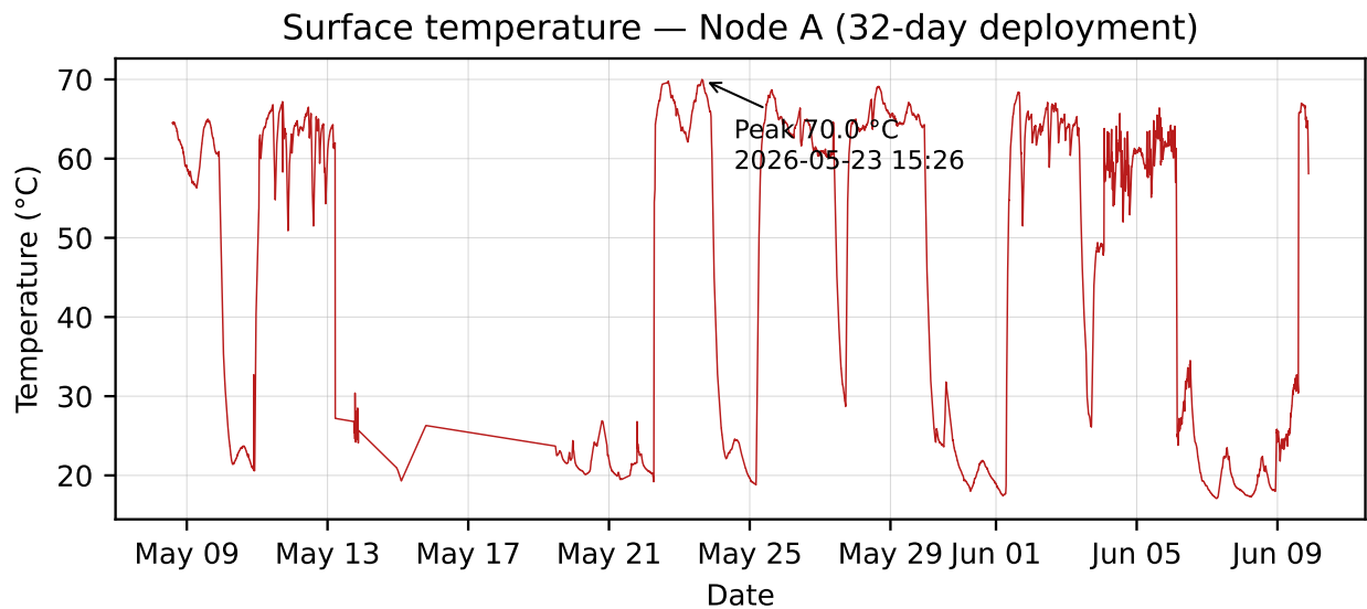
Figure 7: Node A surface-temperature history during the 32-day pilot deployment. The 70.0 °C peak is a historical observation; its annotation does not identify a mechanical cause.
