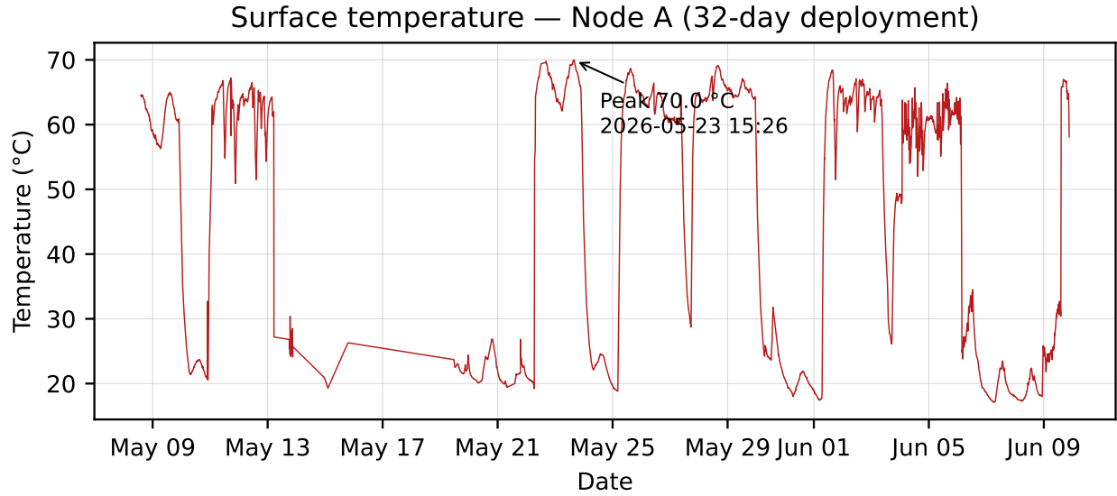
Figure 5: Surface temperature of one node over the 32-day deployment, showing the maximum associated with the suction-fan case.
