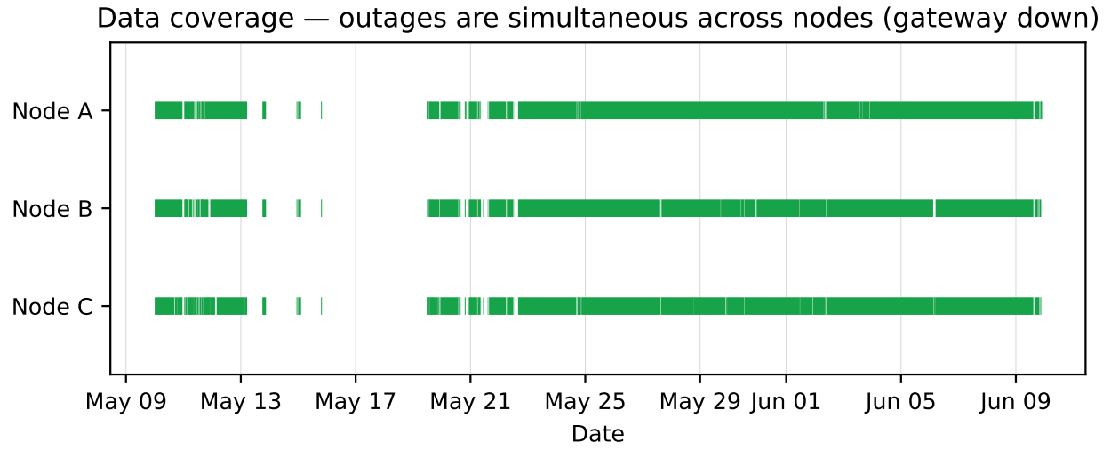
Figure 6: Data coverage of the three nodes. Outages are simultaneous across nodes, corresponding to gateway-off periods rather than LoRa link failures.
