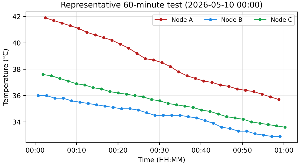
Figure 3: Representative 60-minute window (three nodes active) showing temperature versus time during a night-time cool-down of the machines.
