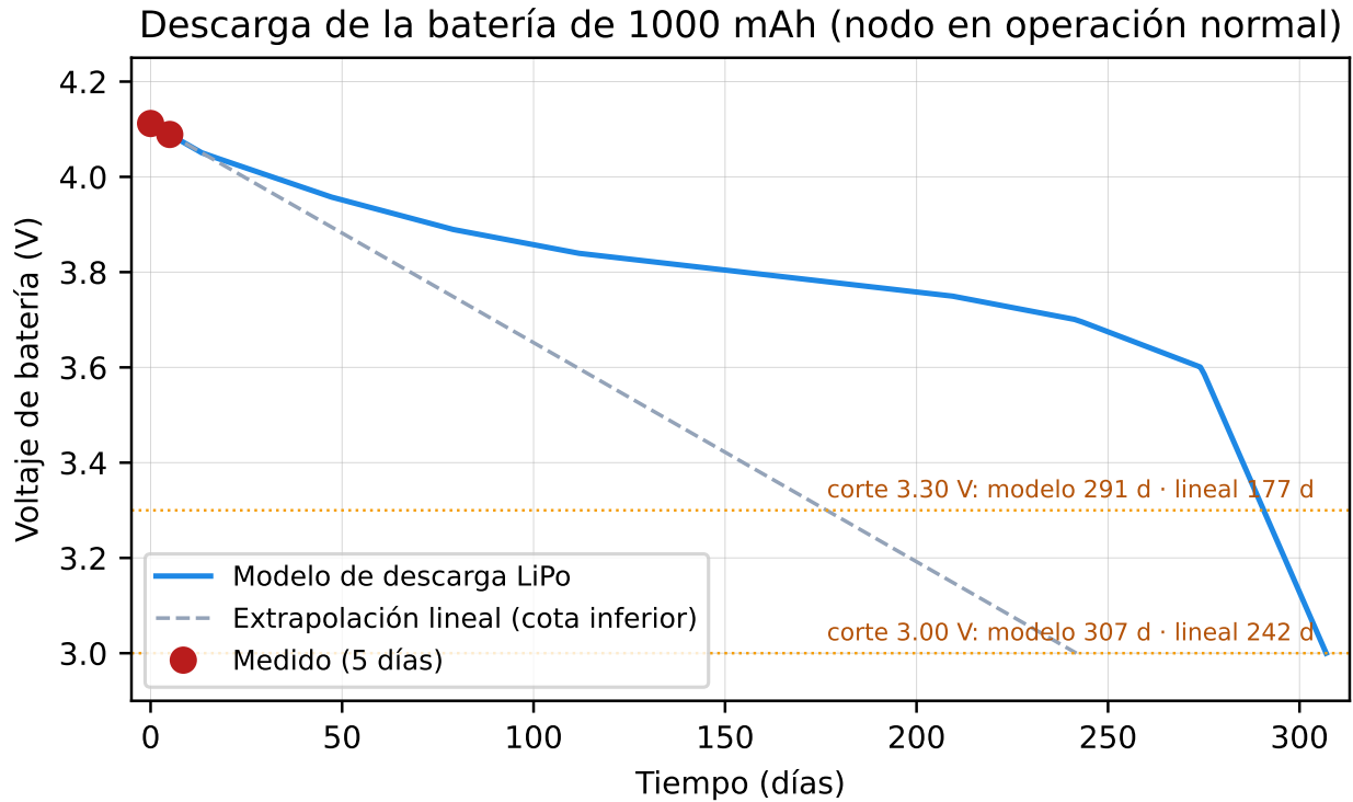
Figure 4: Battery discharge test (1000 mAh cell): measured points, non-linear LiPo discharge model (voltage–state-of-charge curve) and a linear extrapolation as a conservative lower bound. The model estimates an autonomy of about 10 months.
