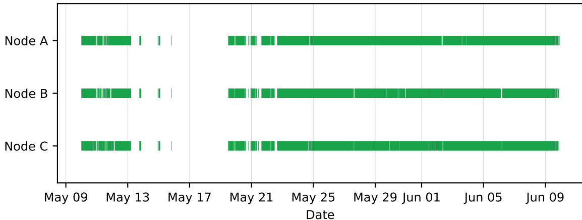
Data coverage — outages are simultaneous across nodes (gateway down)
