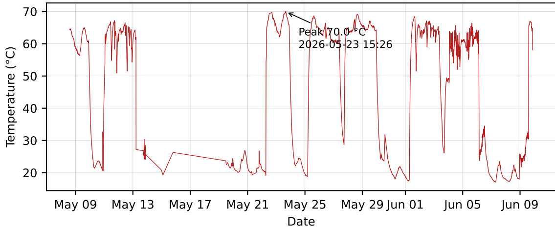
Surface temperature — Node A (32-day deployment)
