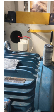
Figure 1: Assembled sensor node mounted on a motor housing: the PT100 probe with the MAX31865 module (left) and the node enclosure with the LoRa antenna (right).
