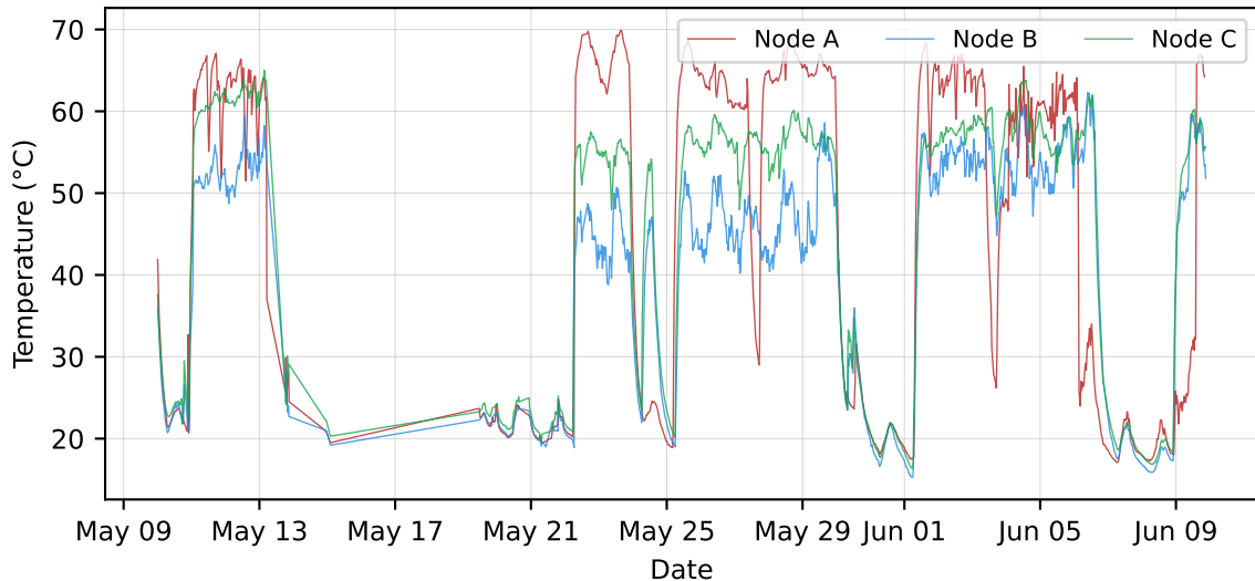
Surface temperature of the three nodes (common window)
