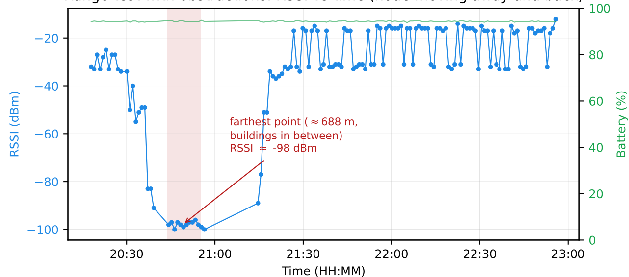
Range test with obstructions: RSSI vs time (node moving away and back)
