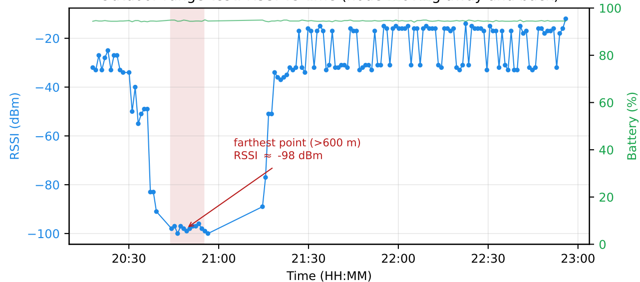
Outdoor range test: RSSI vs time (node moving away and back)
