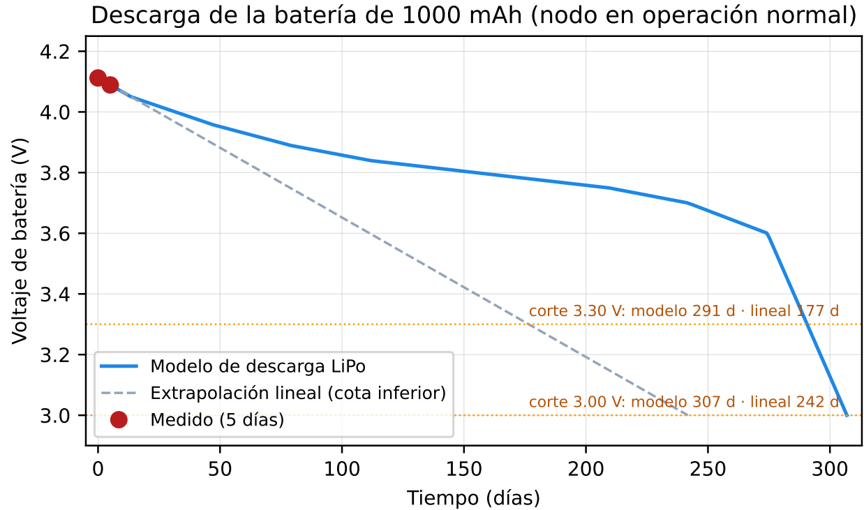
Figure 6: Two measured voltage points over five days with a 1000 mAh cell and extrapolated curves. Estimated autonomy is 177 days (linear, 3.30 V cutoff) or 291–307 days (assumed LiPo curve, 3.30/3.00 V cutoffs). The original plot’s lower-bound label compares models; it does not guarantee service lifetime.
