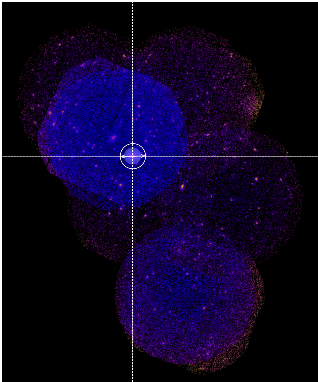
SDSSXCS-64824 - Combined 0.5-2.0keV ratemap
