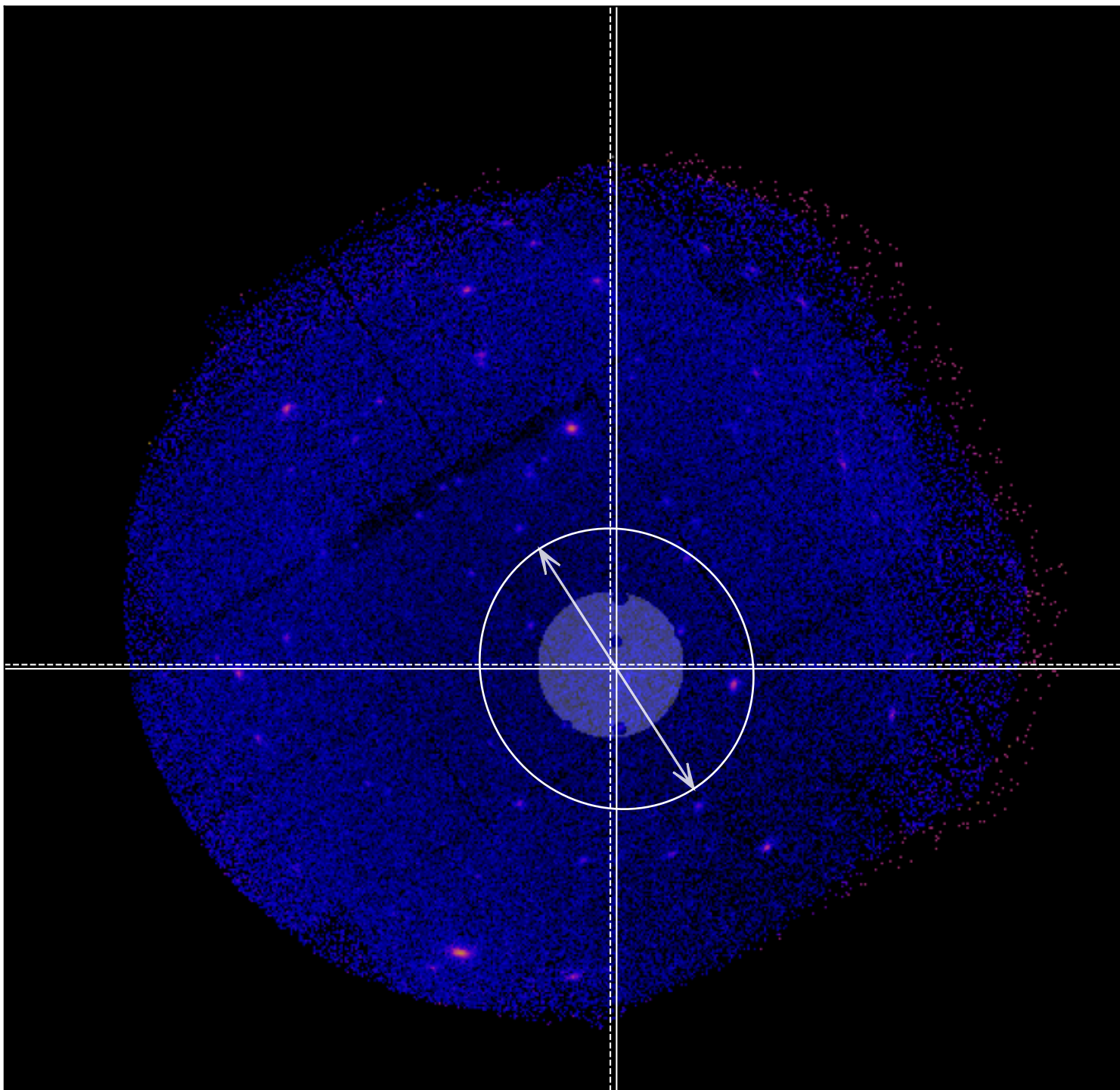
SDSSXCS-26424 - Combined 0.5-2.0keV ratemap
