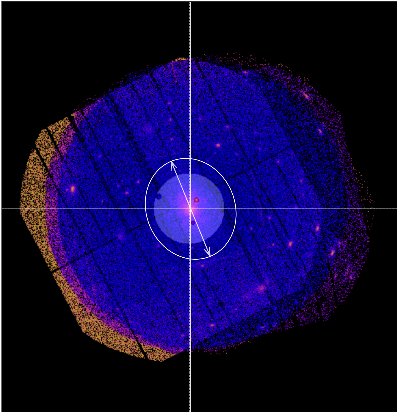
SDSSXCS-5527 - Combined 0.5-2.0keV ratemap
