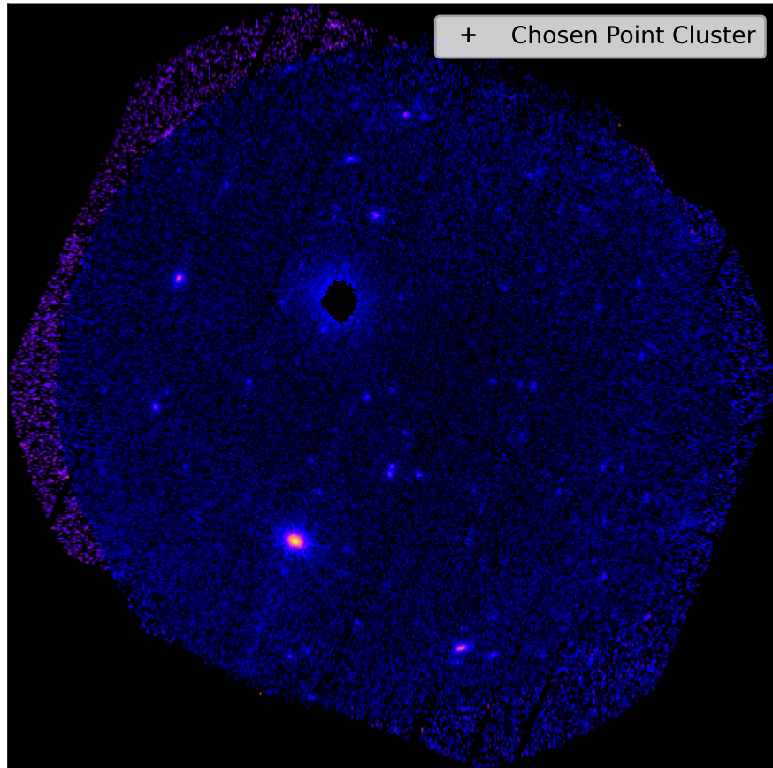
SDSSXCS-1018 - Combined 0.5-2.0keV ratemap
