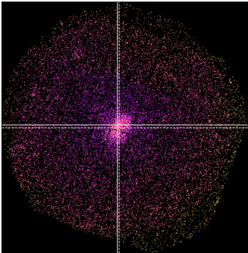
SDSSXCS-119 - Combined 0.5-2.0keV ratemap
