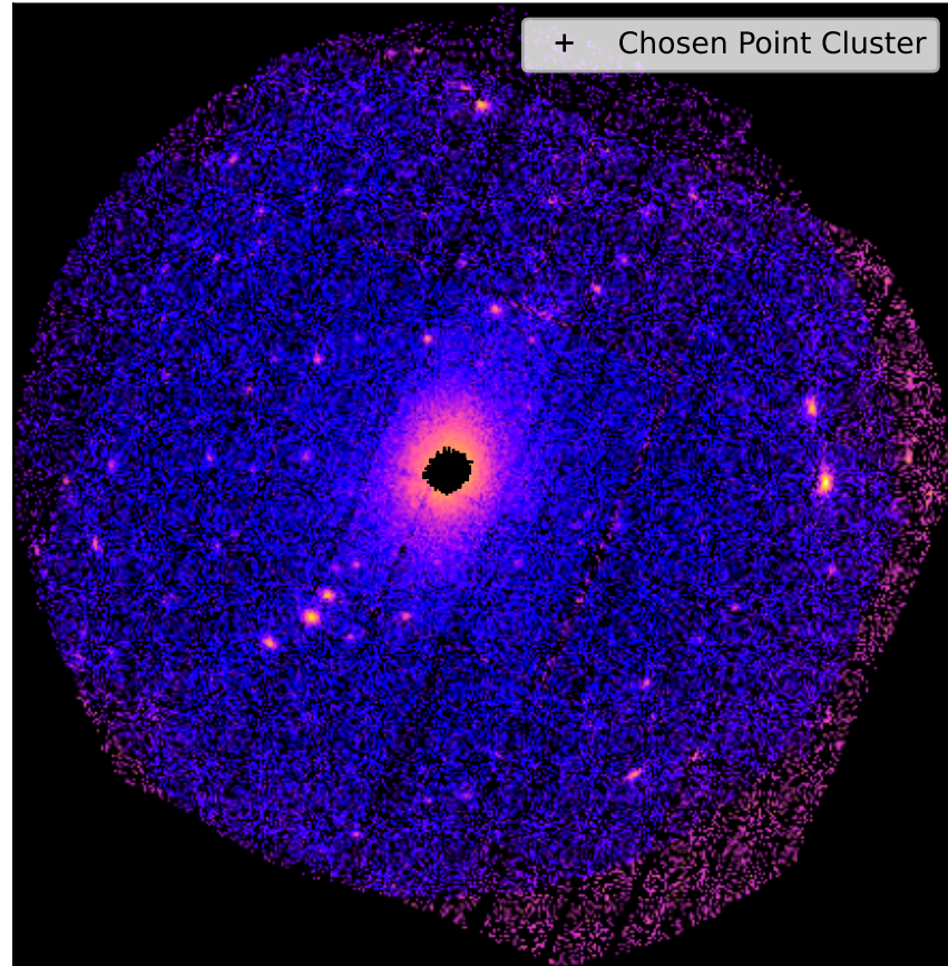
SDSSXCS-124 - Combined 0.5-2.0keV ratemap
