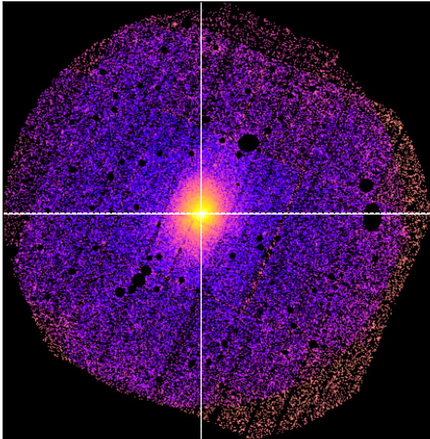
SDSSXCS-124 - Combined 0.5-2.0keV ratemap
