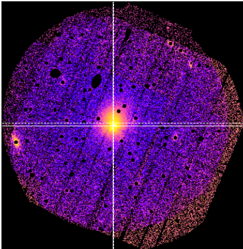
SDSSXCS-134 - Combined 0.5-2.0keV ratemap
