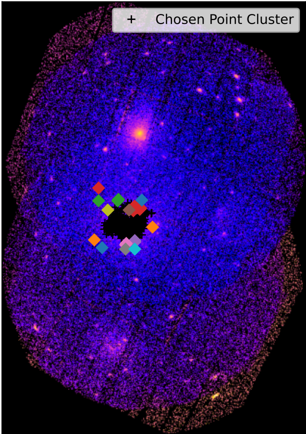
SDSSXCS-15 - Combined 0.5-2.0keV ratemap
