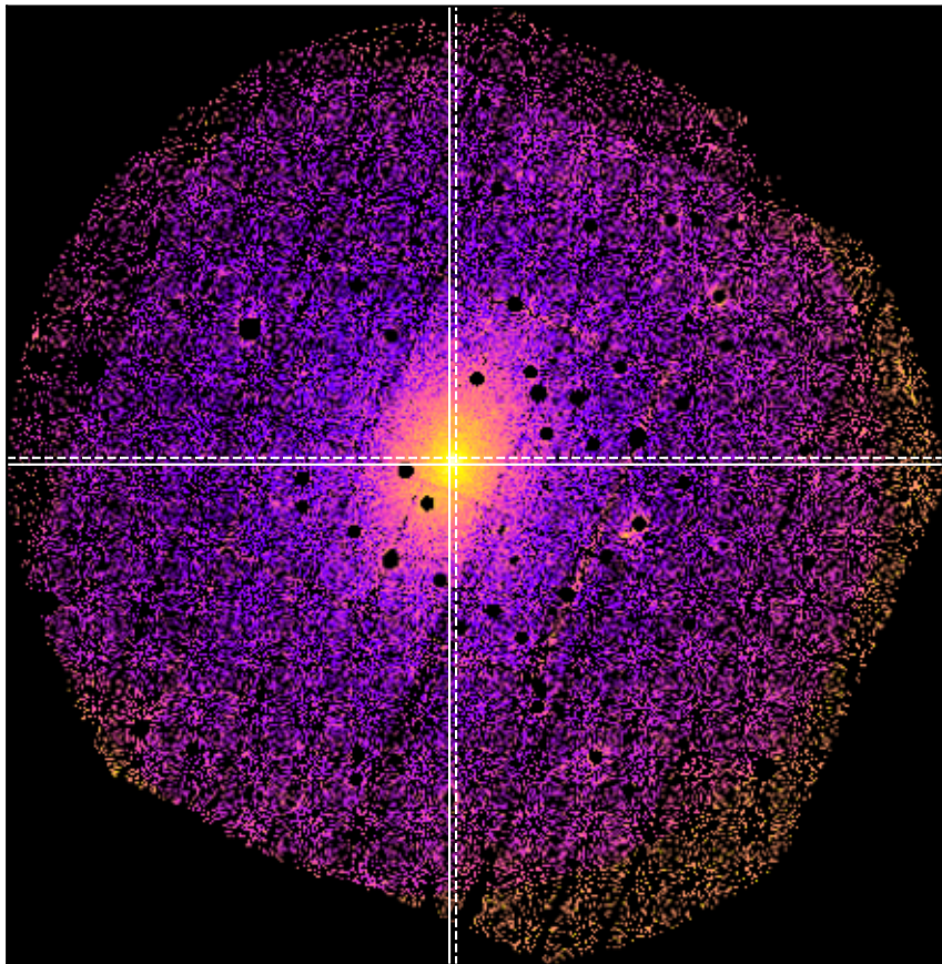
SDSSXCS-2789 - Combined 0.5-2.0keV ratemap
