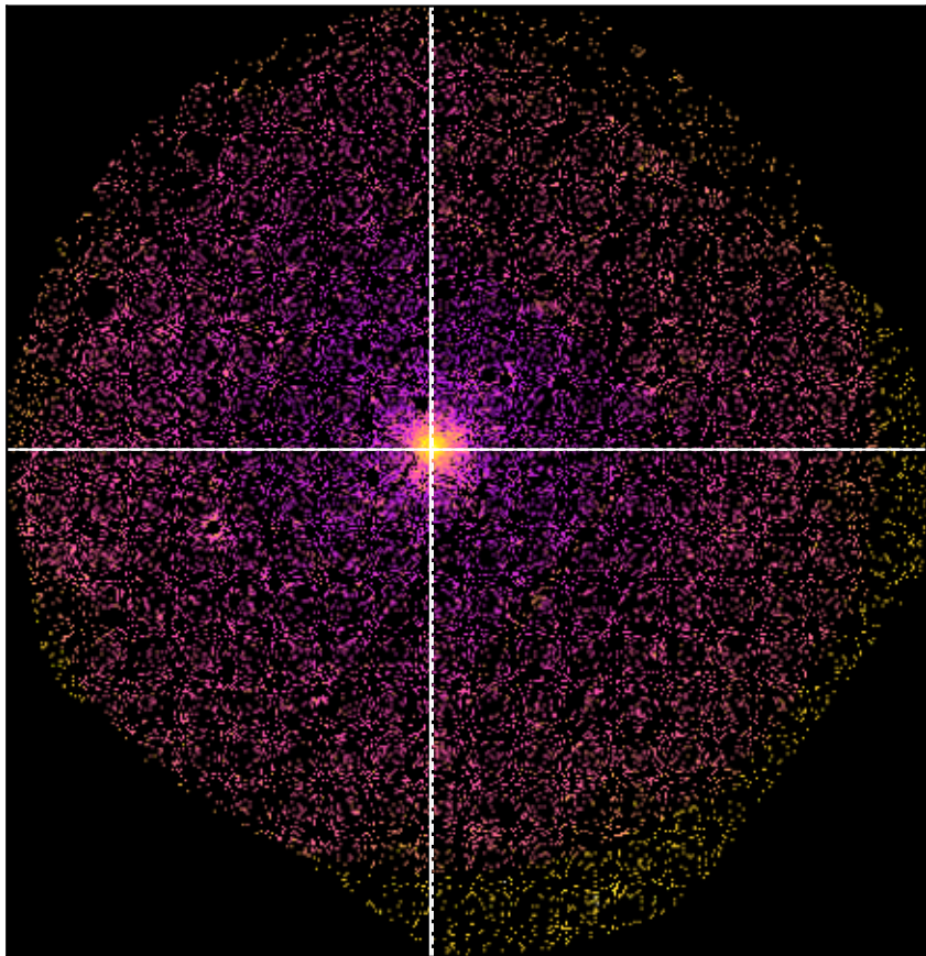
SDSSXCS-290 - Combined 0.5-2.0keV ratemap
