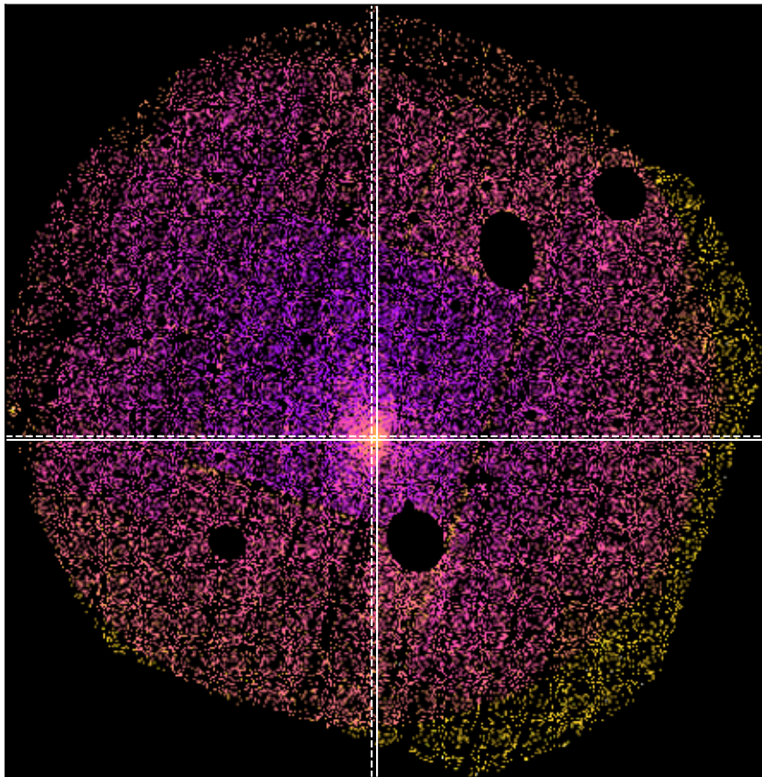
SDSSXCS-5020 - Combined 0.5-2.0keV ratemap
