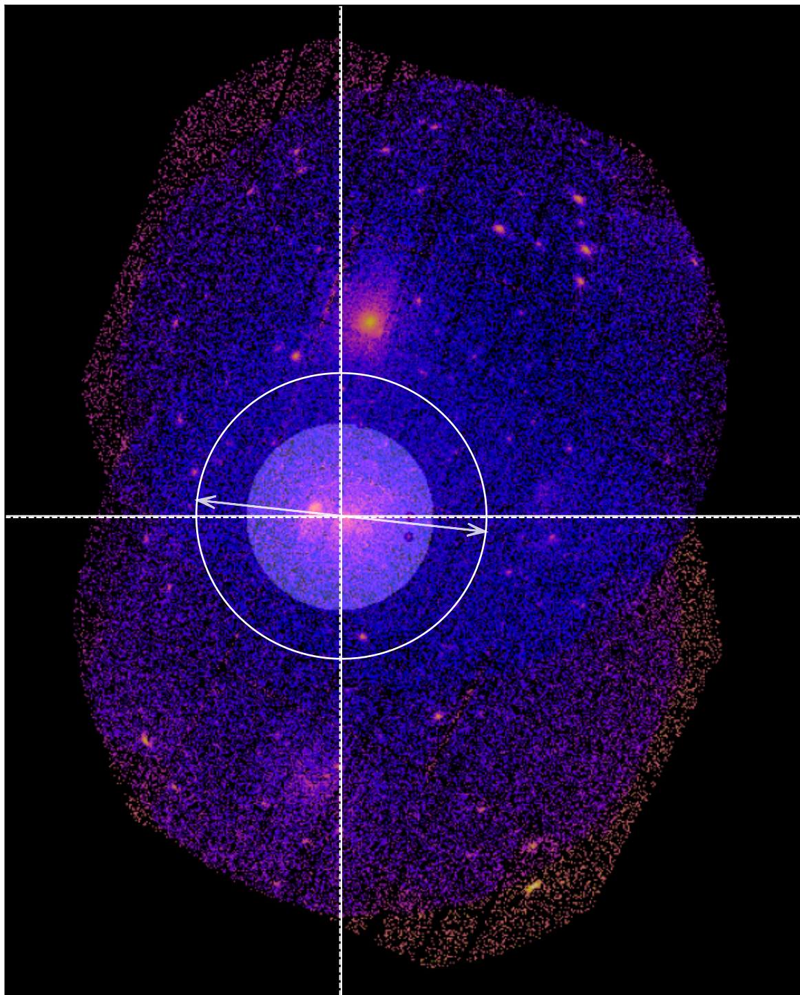
SDSSXCS-15 - Combined 0.5-2.0keV ratemap
