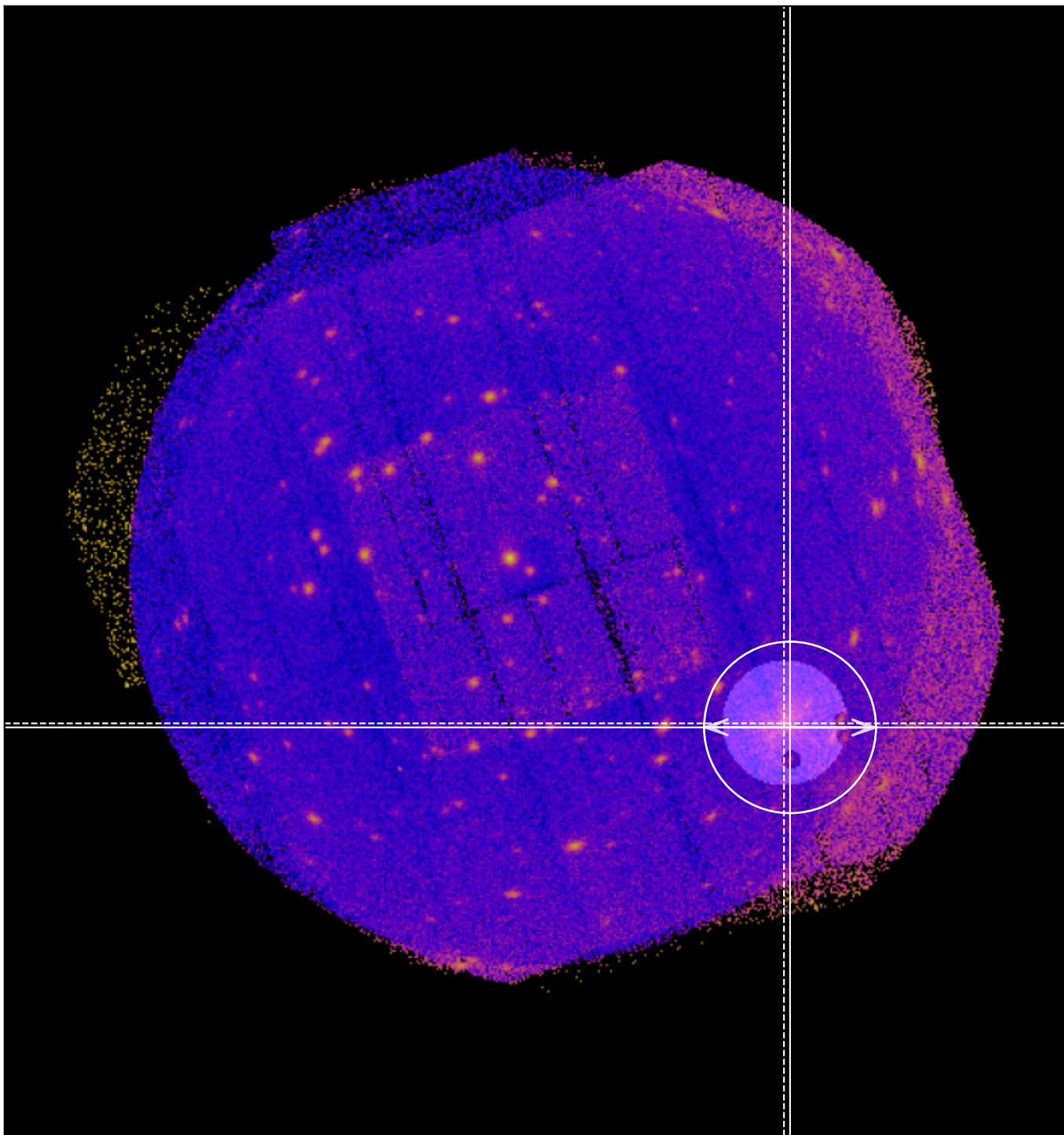
SDSSXCS-21847 - Combined 0.5-2.0keV ratemap
