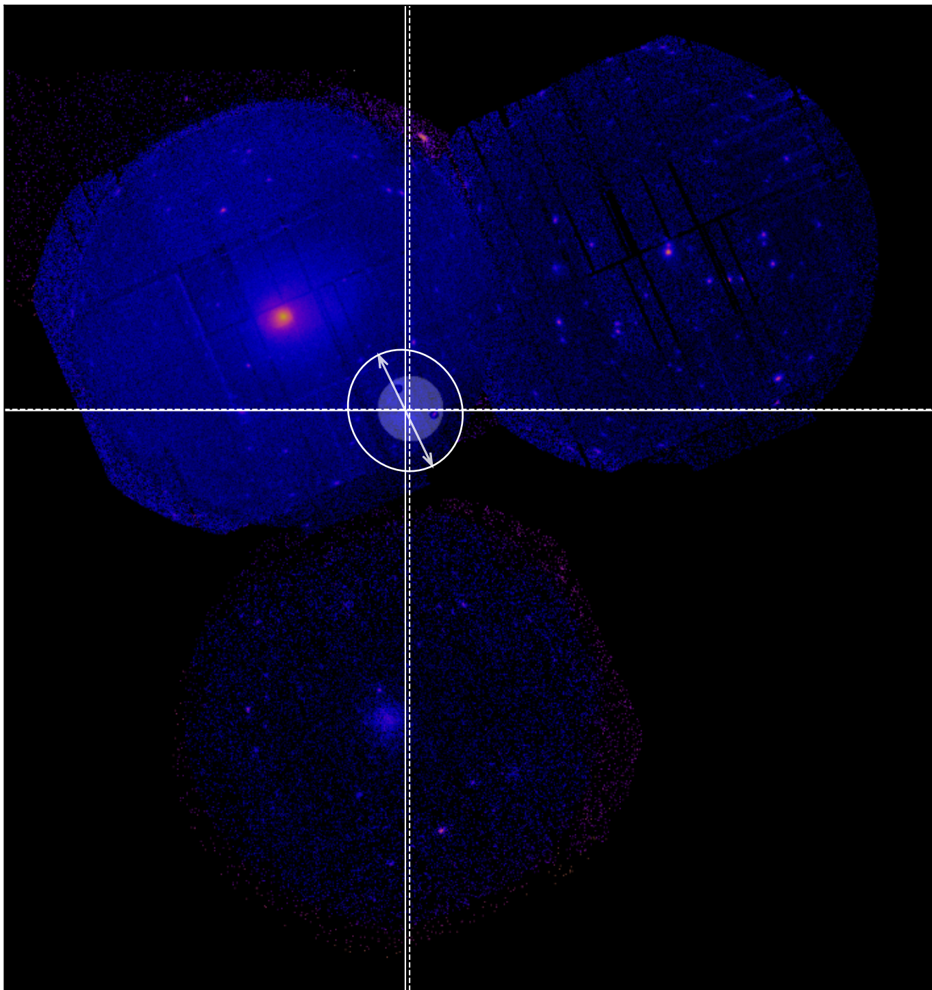
SDSSXCS-474 - Combined 0.5-2.0keV ratemap
