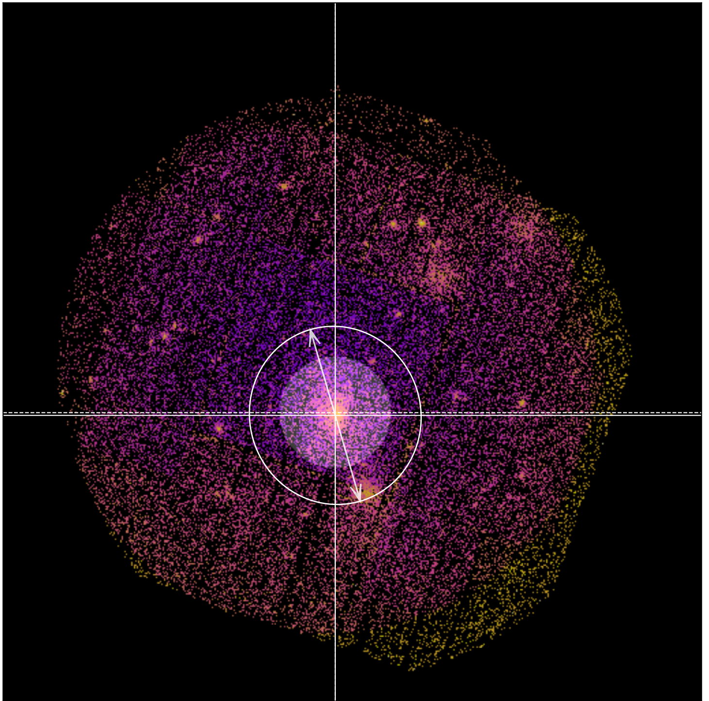
SDSSXCS-5020 - Combined 0.5-2.0keV ratemap
