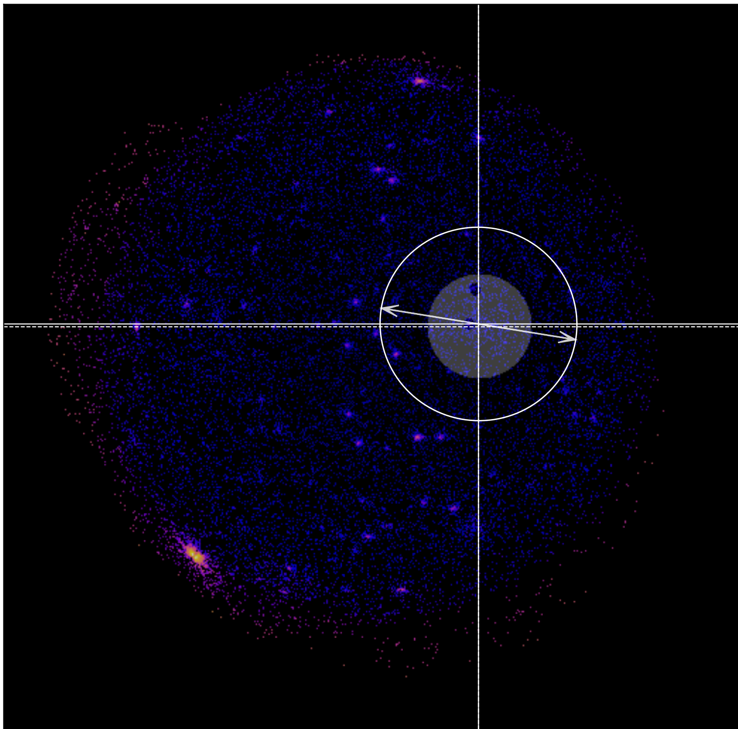
SDSSXCS-7247 - Combined 0.5-2.0keV ratemap
