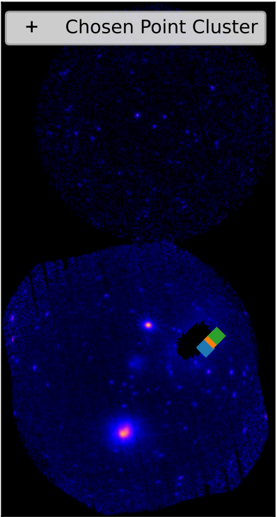
SDSSXCS-103 - Combined 0.5-2.0keV ratemapSDSSXCS-103 - Combined 0.5-2.0keV ratemap
