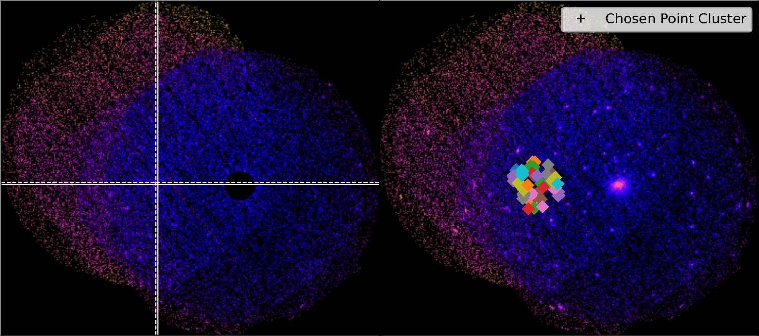
SDSSXCS-10897 - Combined 0.5-2.0keV ratemapSDSSXCS-10897 - Combined 0.5-2.0keV ratemap
