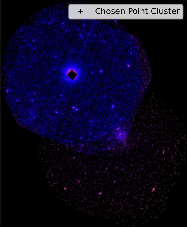
SDSSXCS-11331 - Combined 0.5-2.0keV ratemap
