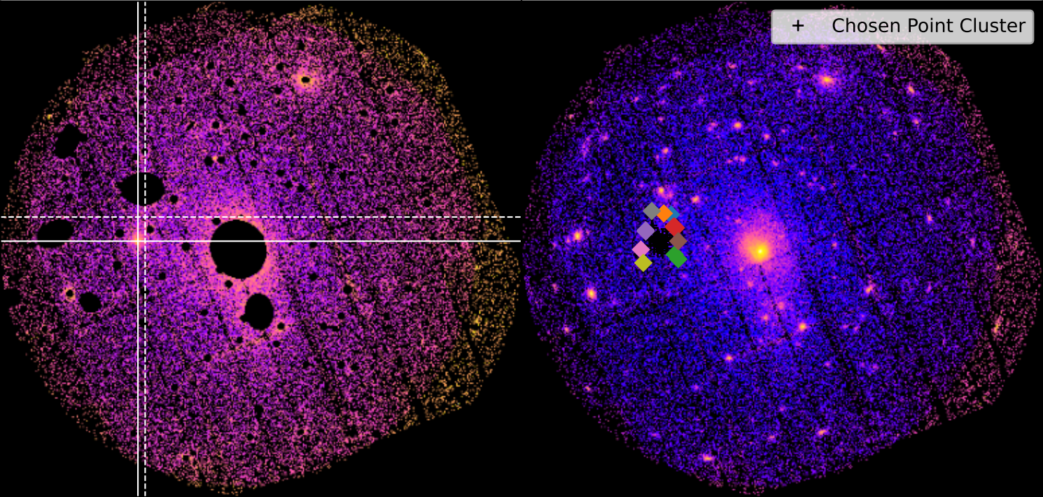
SDSSXCS-11394 - Combined 0.5-2.0keV ratemapSDSSXCS-11394 - Combined 0.5-2.0keV ratemap
