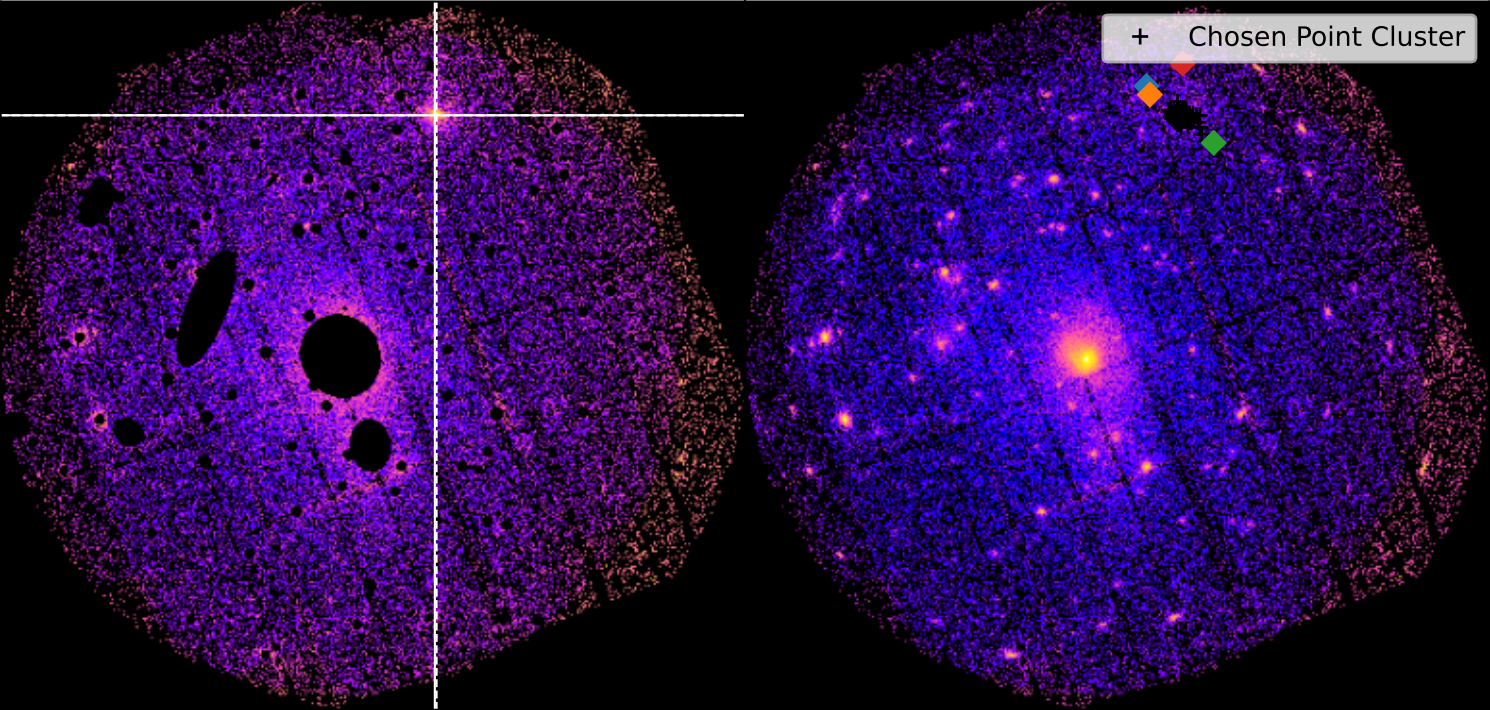
SDSSXCS-11881 - Combined 0.5-2.0keV ratemapSDSSXCS-11881 - Combined 0.5-2.0keV ratemap
