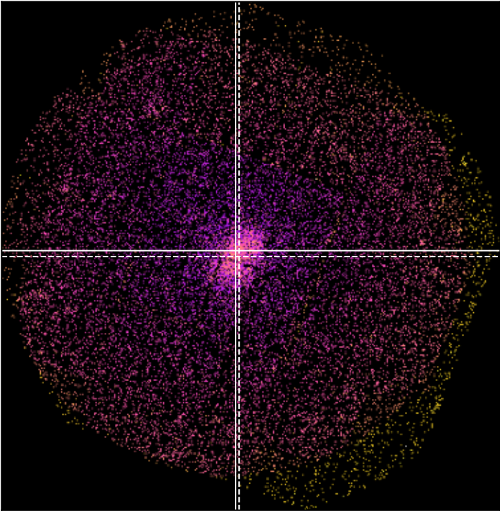
SDSSXCS-119 - Combined 0.5-2.0keV ratemapSDSSXCS-119 - Combined 0.5-2.0keV ratemap
