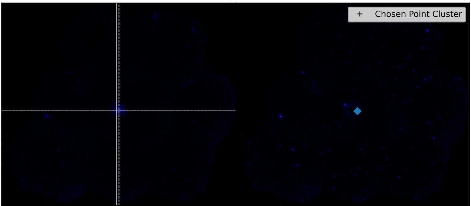
SDSSXCS-120 - Combined 0.5-2.0keV ratemapSDSSXCS-120 - Combined 0.5-2.0keV ratemap
