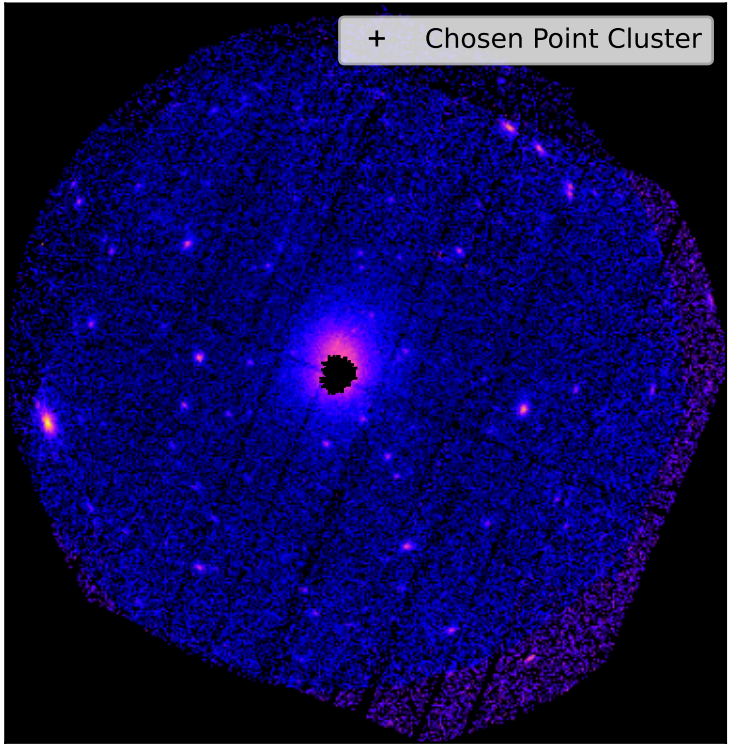
SDSSXCS-134 - Combined 0.5-2.0keV ratemapSDSSXCS-134 - Combined 0.5-2.0keV ratemap
