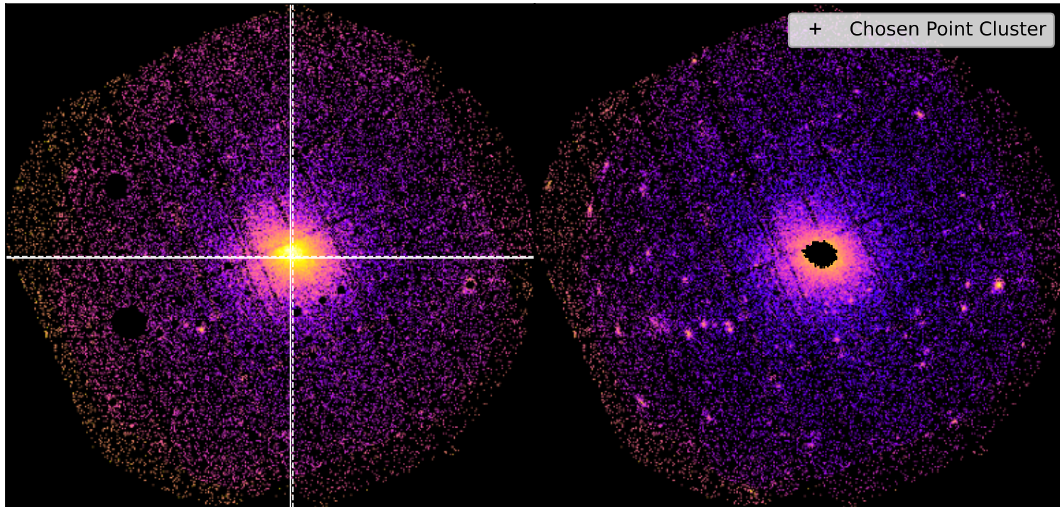
SDSSXCS-13 - Combined 0.5-2.0keV ratemap SDSSXCS-13 - Combined 0.5-2.0keV ratemap
