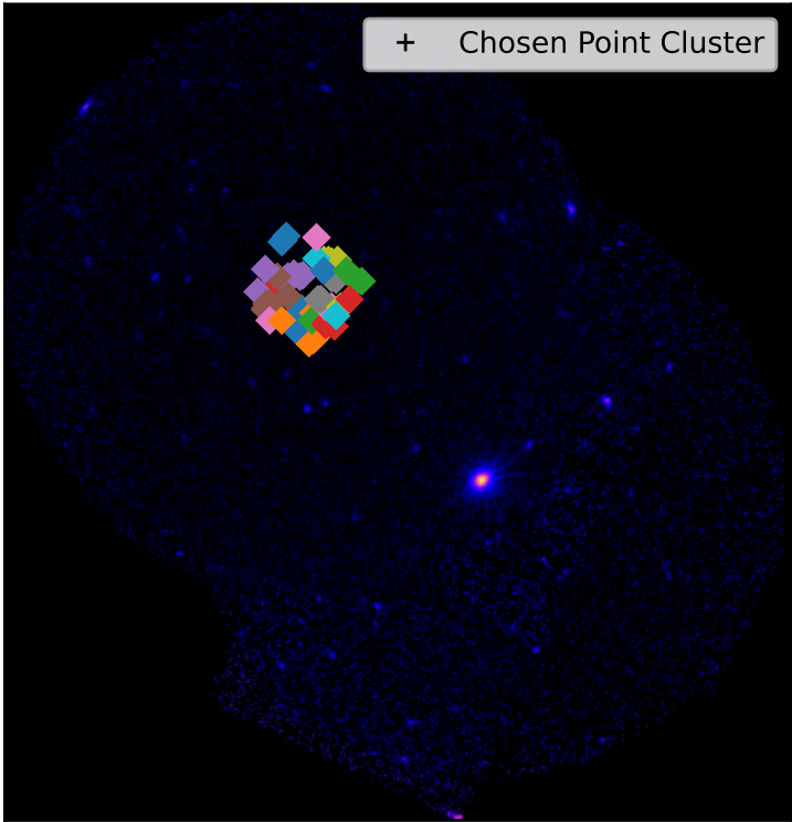
SDSSXCS-14715 - Combined 0.5-2.0keV ratemap
